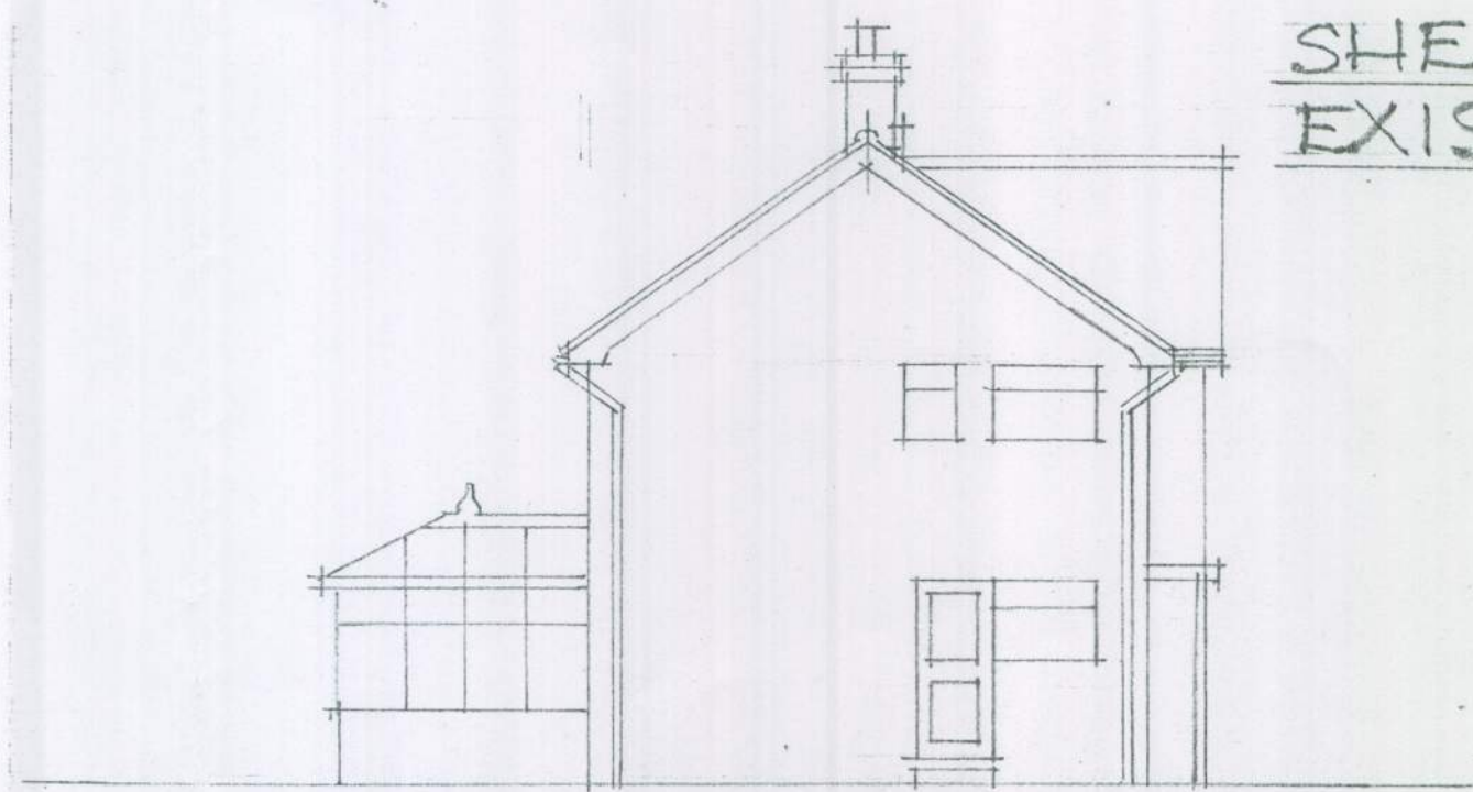
SIDE ELE. (SOUTH) (1:100)
