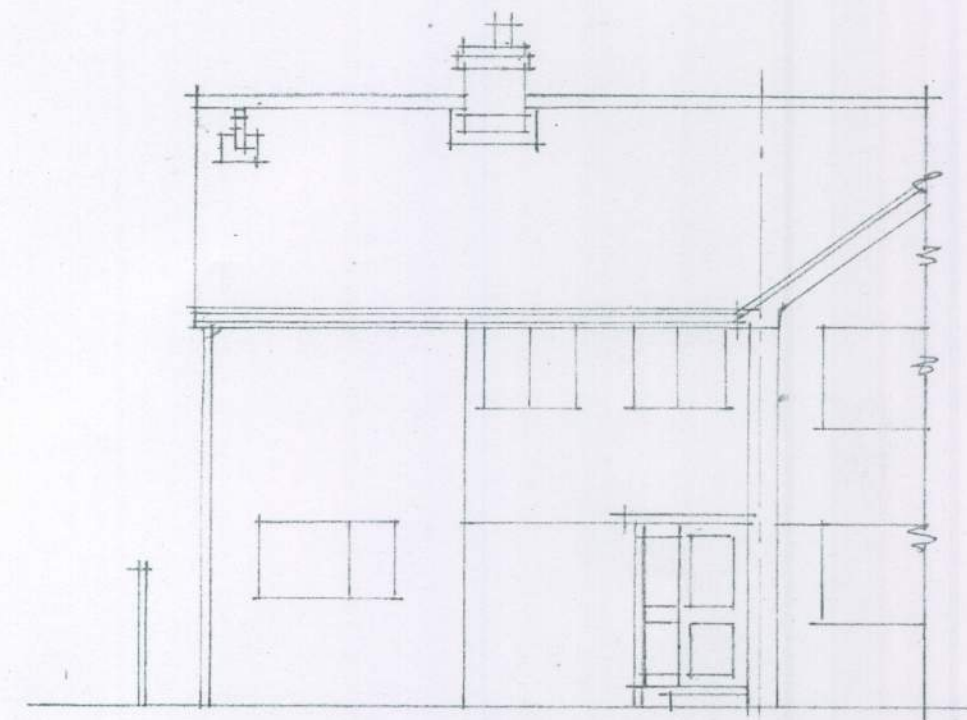
FRONT ELE (EAST) (1:100)
