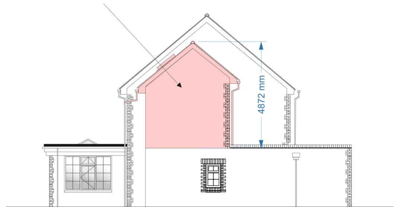
Side elevation showing proposed single story bathroom extension over existing utility room and cloakroom
