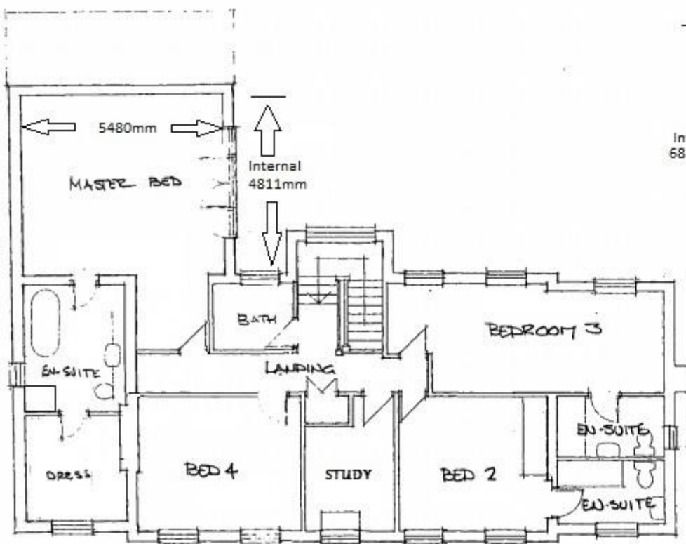
FIRST FLOOR PLAN 1-00
