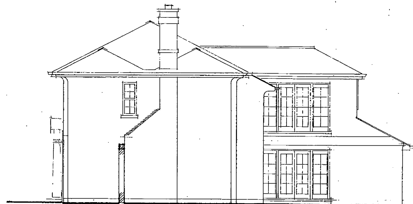
SIDE ELEVATION - EAST 1-100
