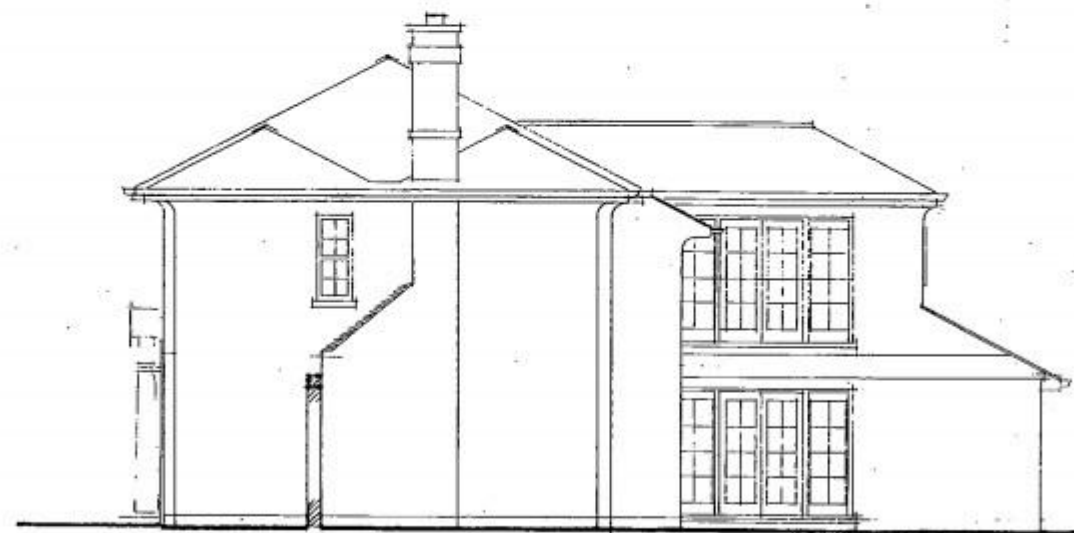
SIDE ELEVATION - EAST 1-100
