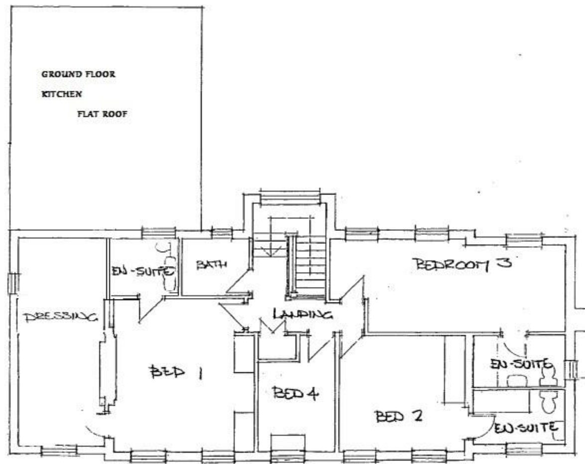
FIRST FLOOR PLAN 1-00
