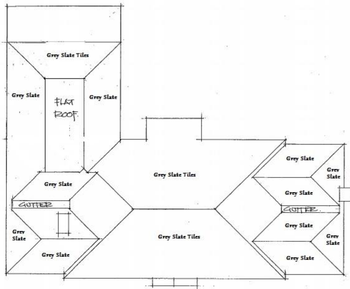
ROOF PLAN PROPOSED 1:100
