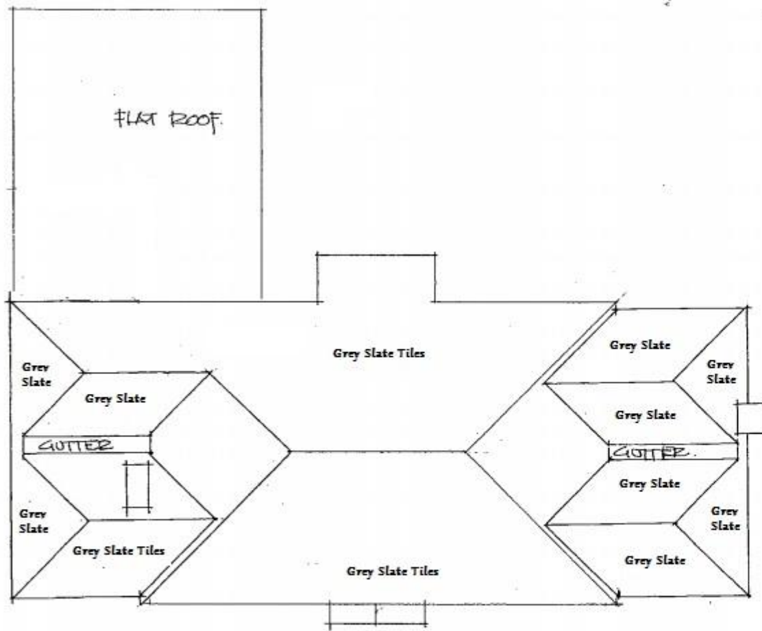
ROOF PLAN EXISTING 1:100
