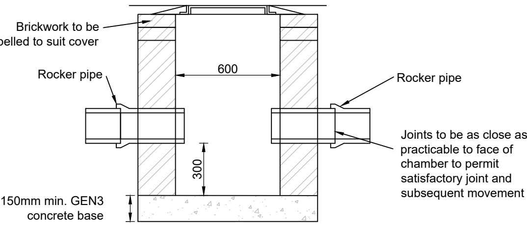
CATCHPIT CHAMBER DETAIL (Scale 1:20)
