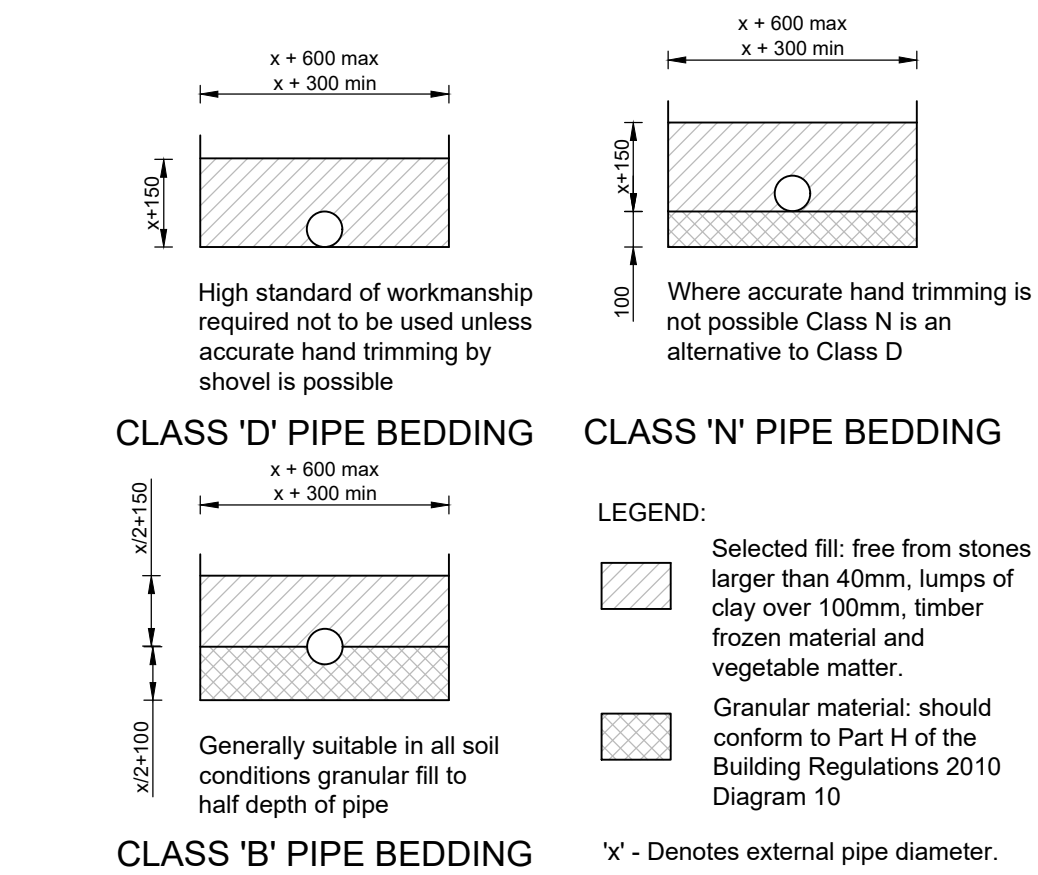
PIPE BEDDING DETAILS (PRIVATE DRAINS) (Scale 1:20)
