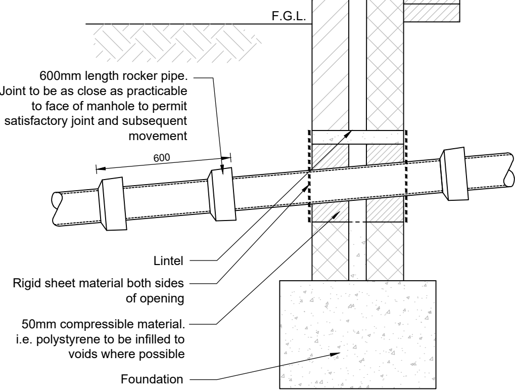
TYPICAL SECTION DETAILING PIPE 'SLEEVE' THROUGH LINTEL OPENING (Scale 1:20)
