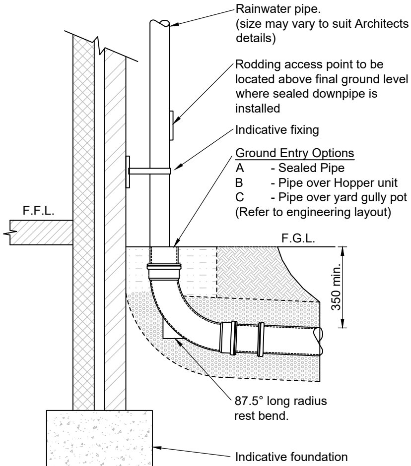
RAINWATER PIPE DETAIL (Scale 1:20)
