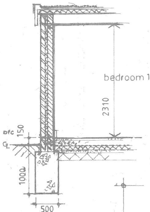
VERTICAL SECTION A — A
