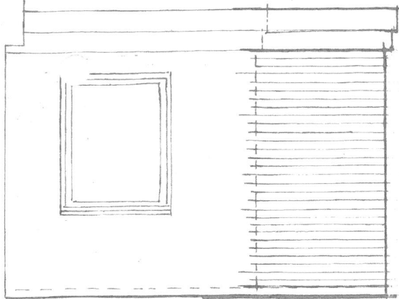
S.E.ELEVATION — AS PROPOSED
