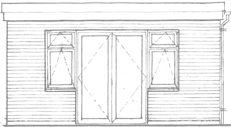
N.W.ELEVATION — AS PROPOSED
