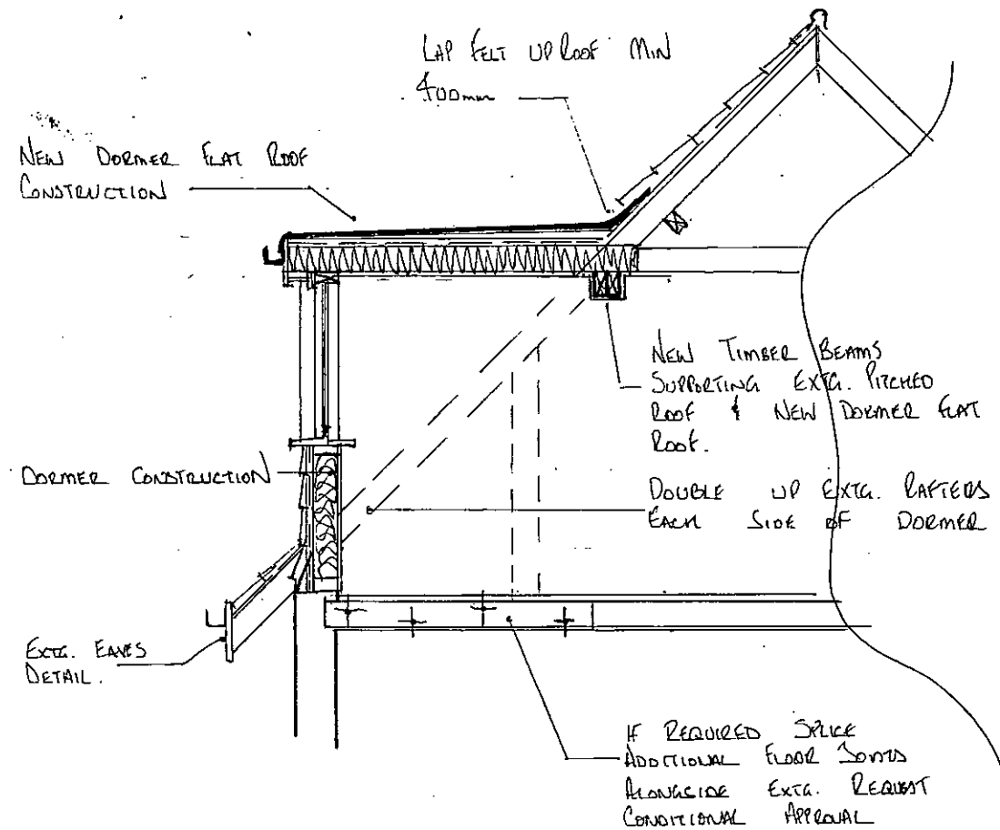
SECTION DETAIL X - X .
