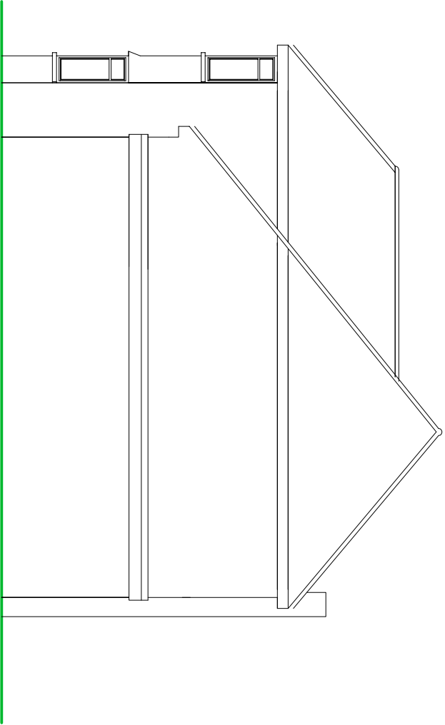
SIDE ELEVATION
