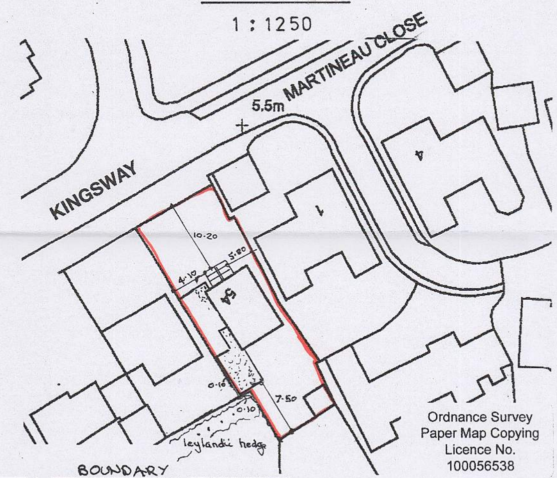
block plan
