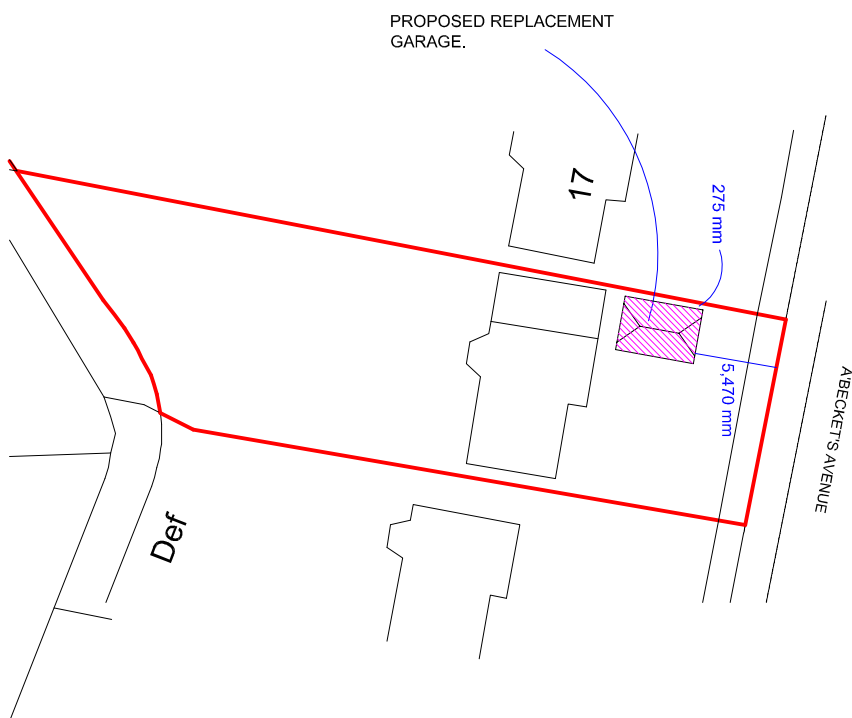
SITE/ROOF PLAN - 1/500
