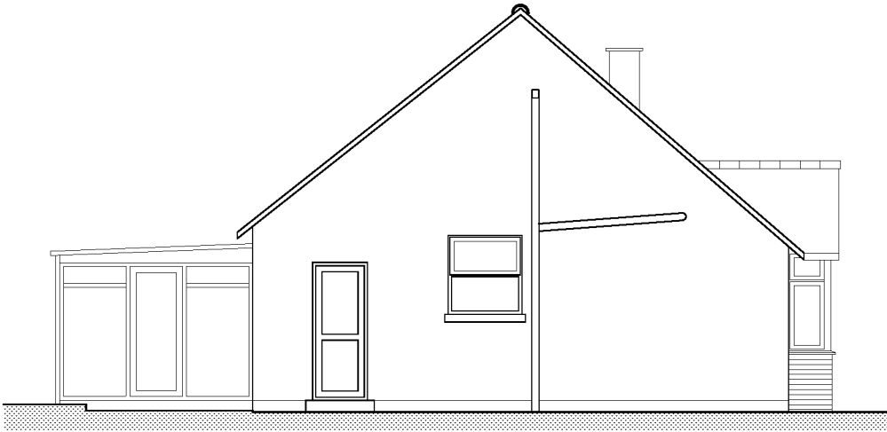
EXISTING SOUTH ELEVATION @ 1:100
