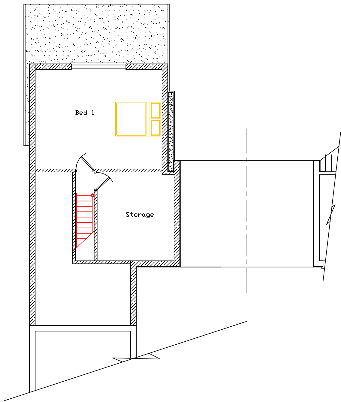
Proposed Loft Floor Plan
