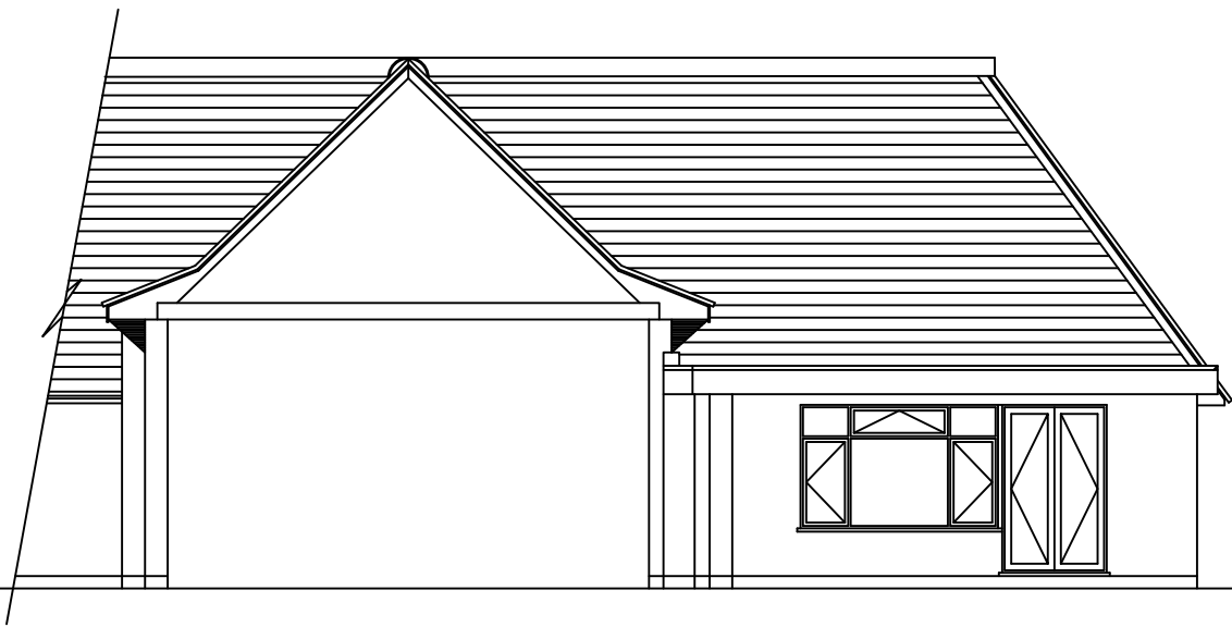
Existing SSW Elevation
