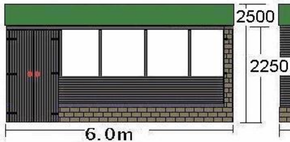
Side
