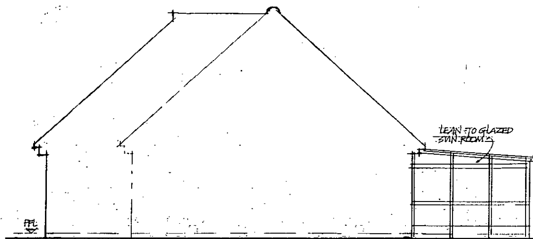
SIDE ELEVATION FROM ADJACENT PROPERTY • 1:100 (A/A-3)
