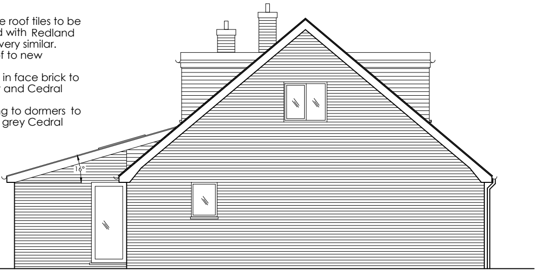
SIDE ELEVATION
