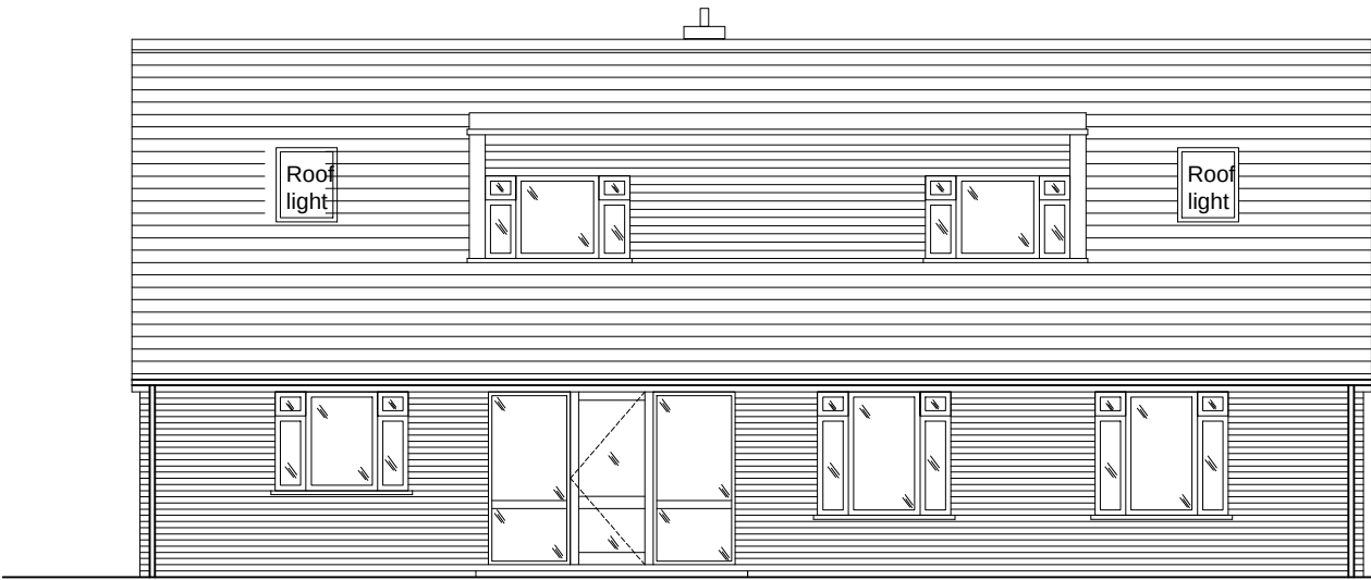
FRONT ELEVATION
