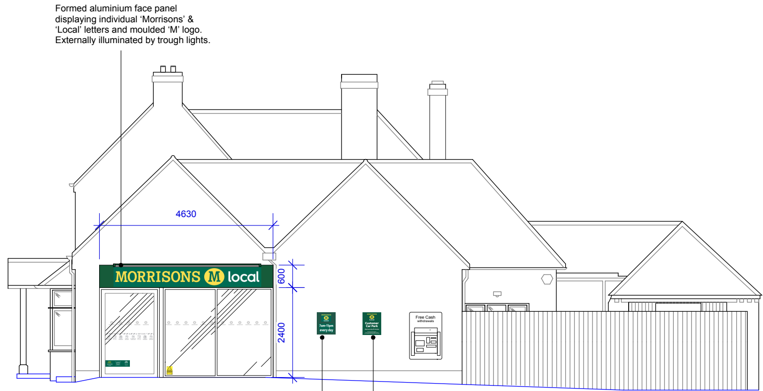
FRONT ELEVATION
