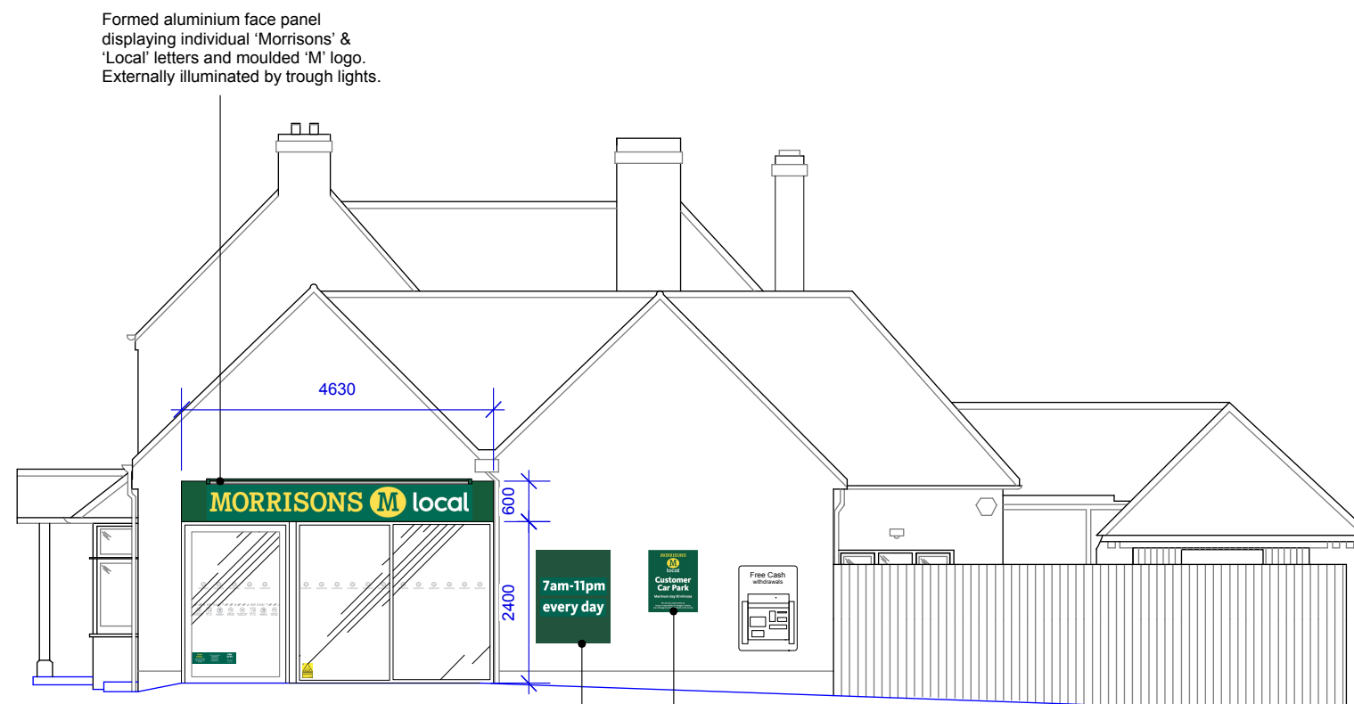
FRONT ELEVATION
