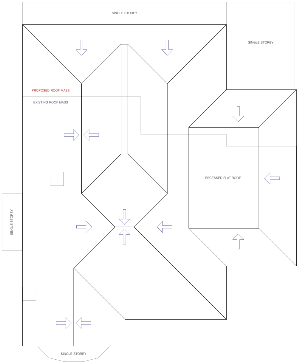
Proposed Roof Plan at 1:100 scale
