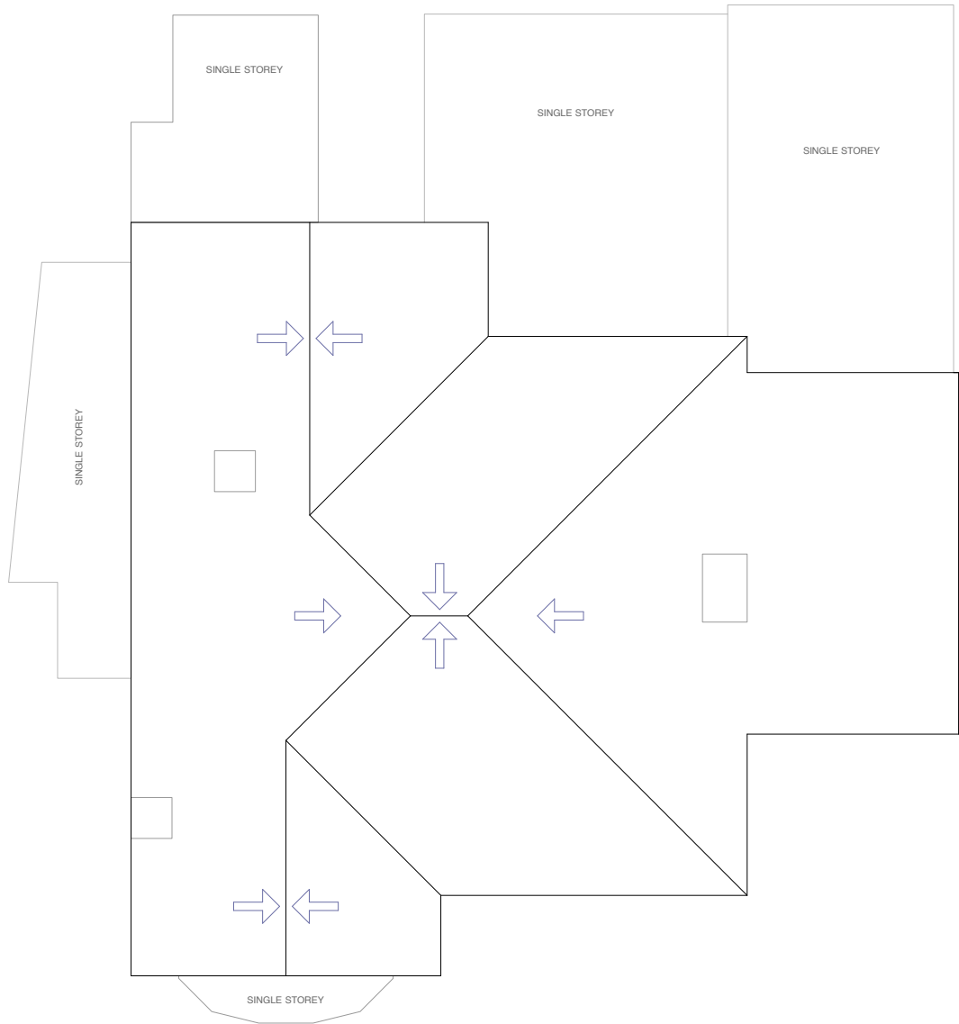
Existing Roof Plan at 1:100 scale
