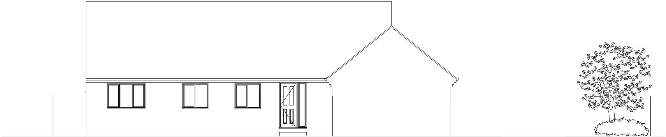
EASTERN ELEVATION
