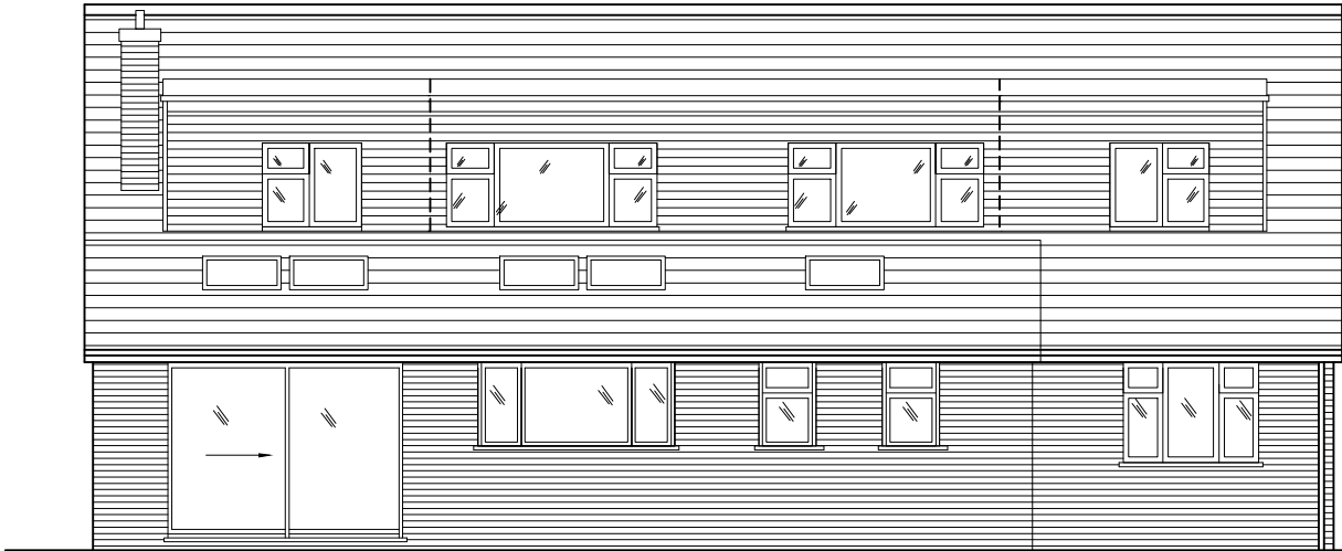
BACK ELEVATION
