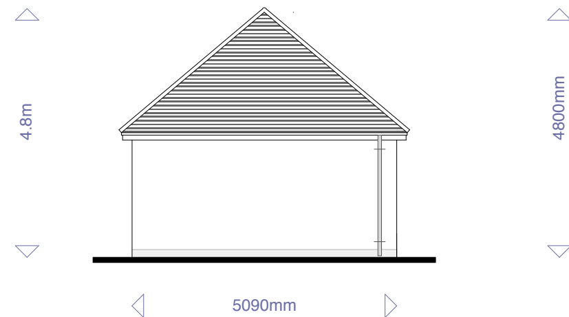
Proposed Rear Elevation at 1:100 scale
