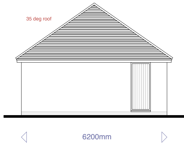
Proposed Side Elevation at 1:100 scale
