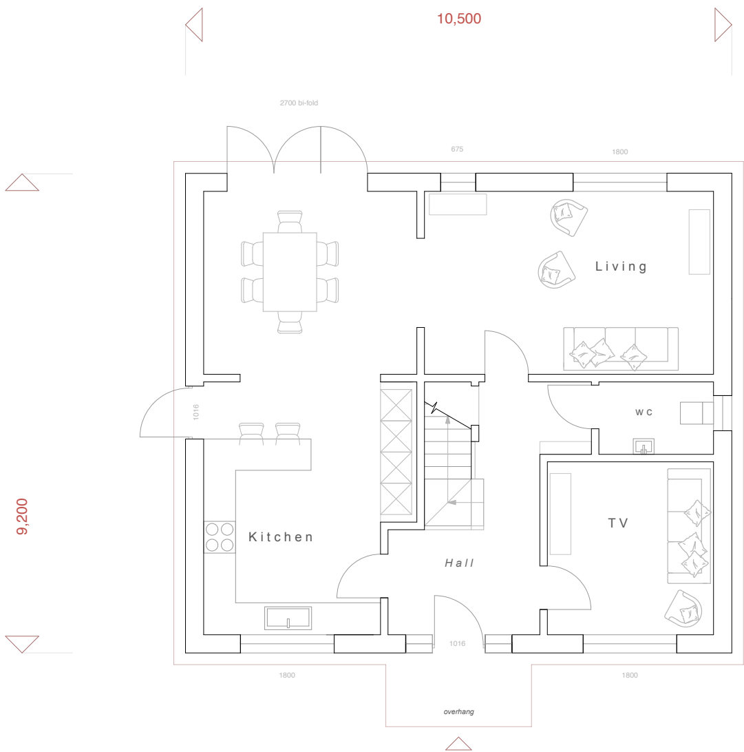
Proposed GF Plan at 1:100 scale
