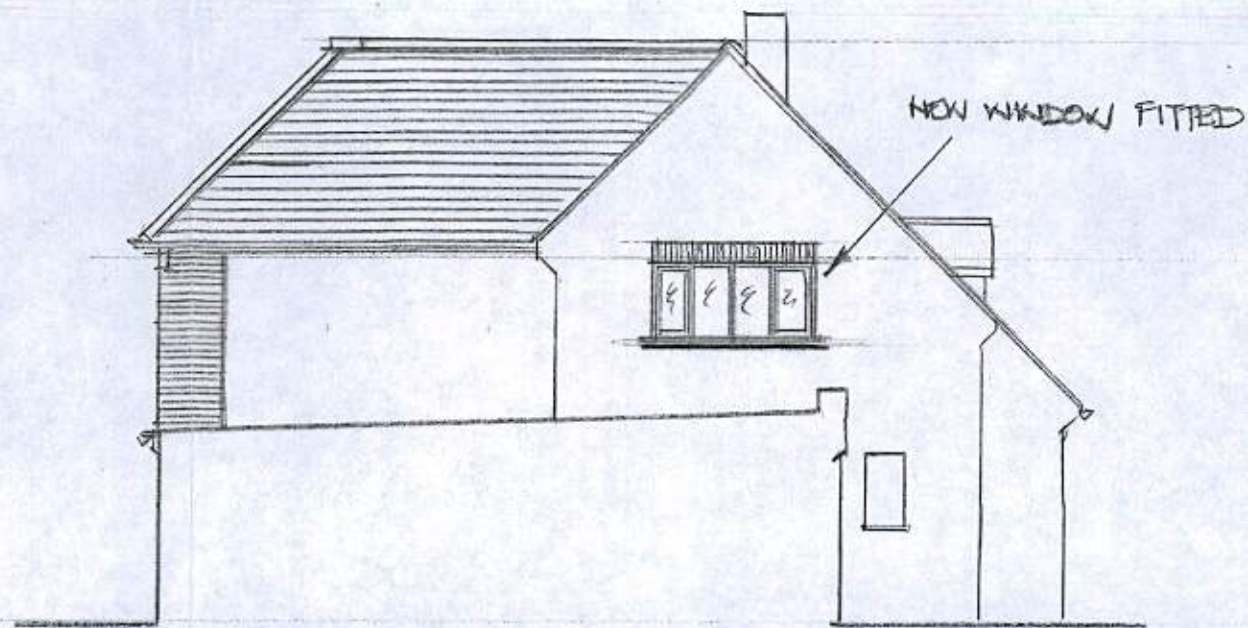
AS BUILT FOR S.W. ELEVATION (Awaiting Approval, Retrospective application)
