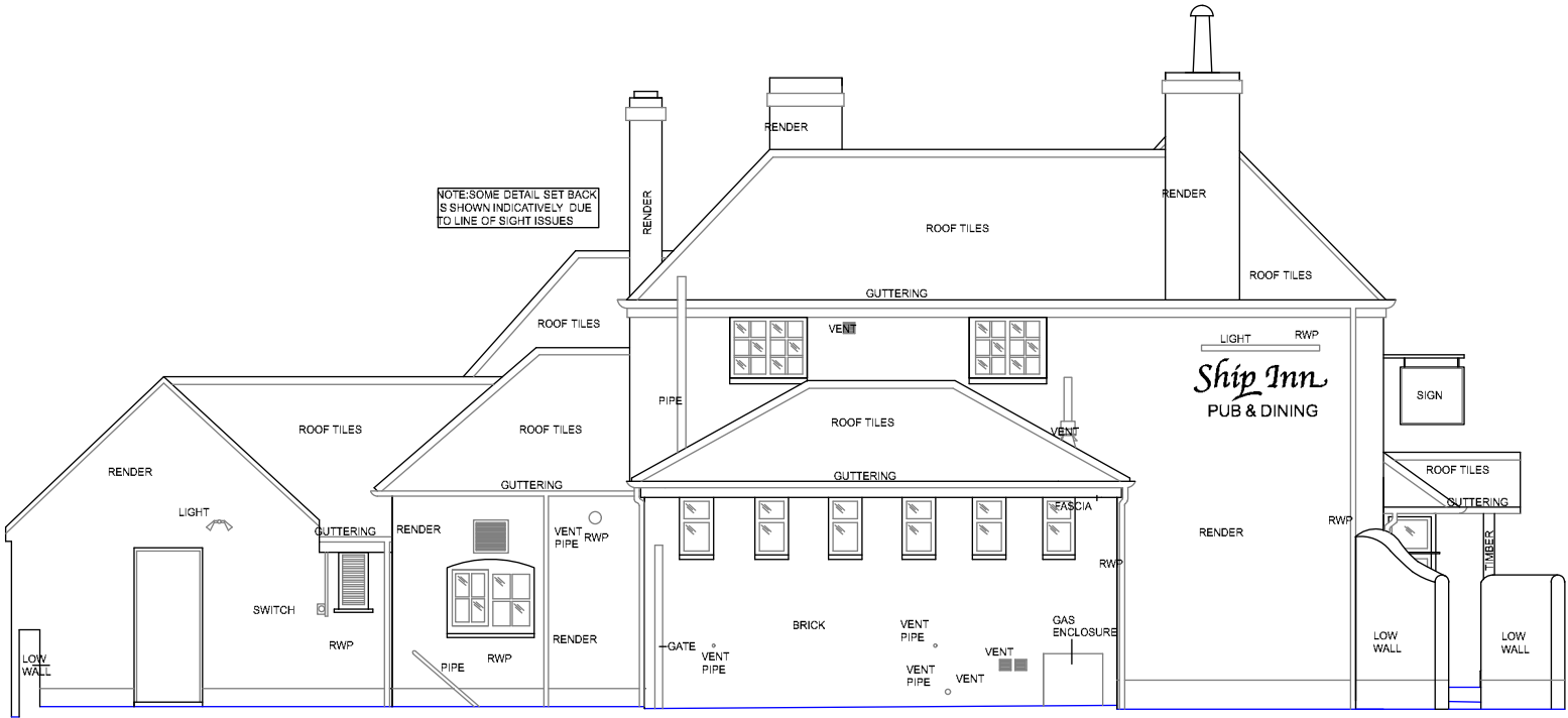
SIDE ELEVATION
