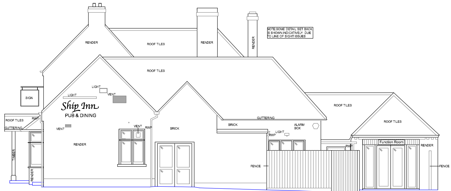
SIDE ELEVATION
