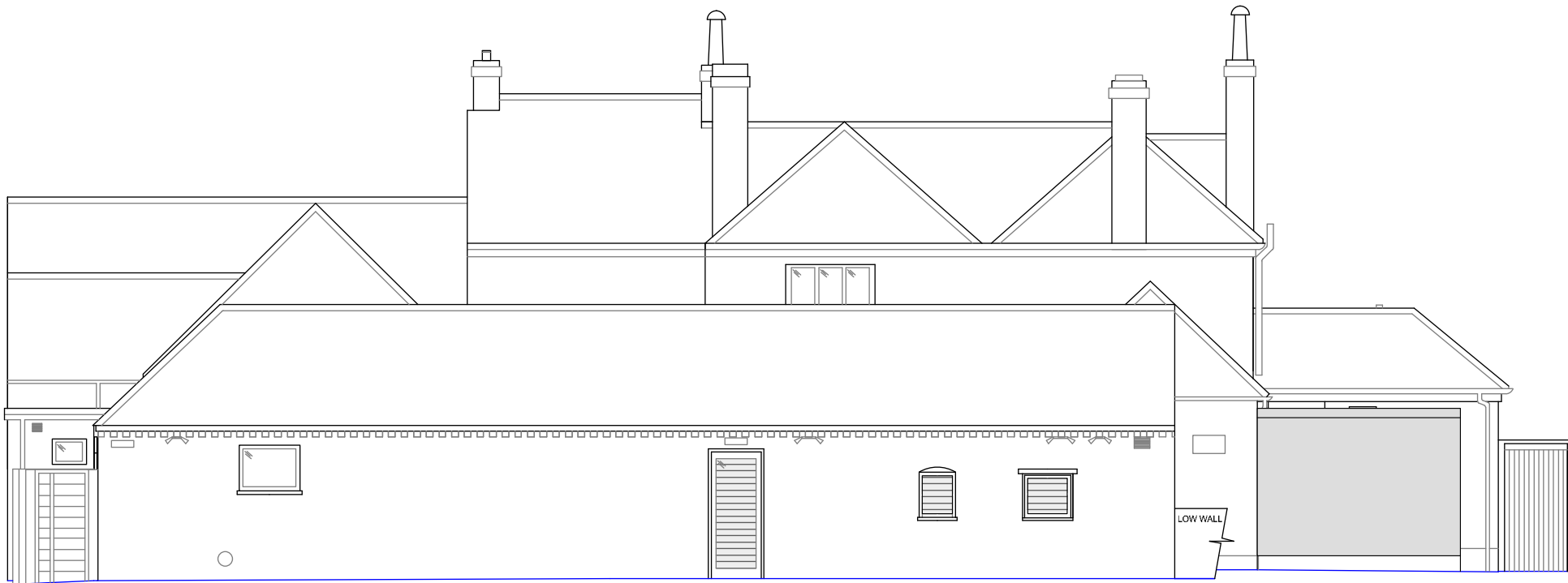
REAR ELEVATION
