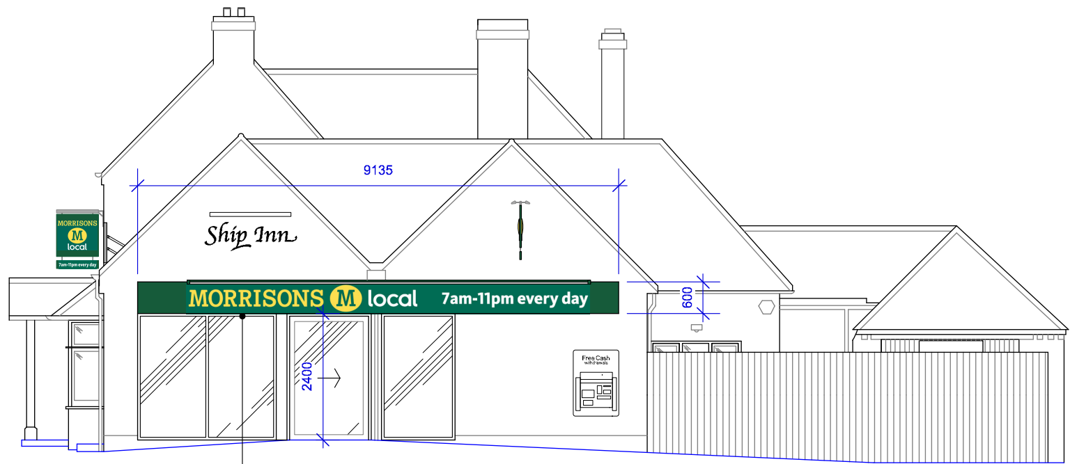
SIDE ELEVATION
