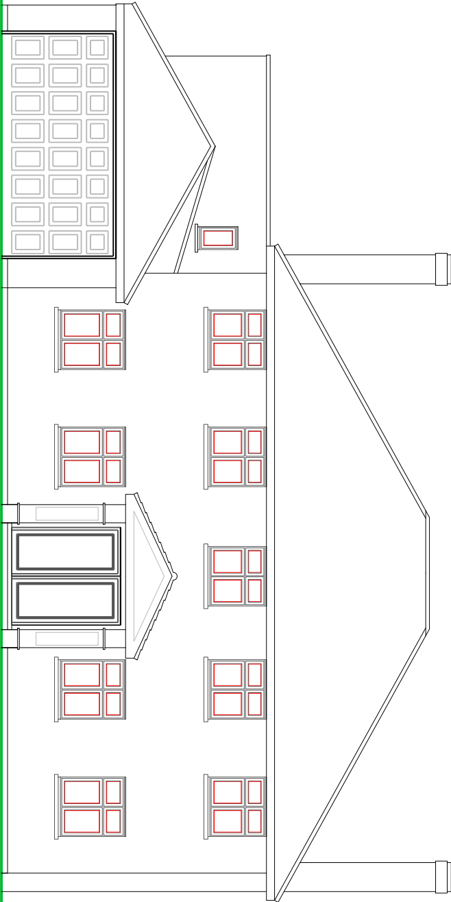
FRONT ELEVATION
