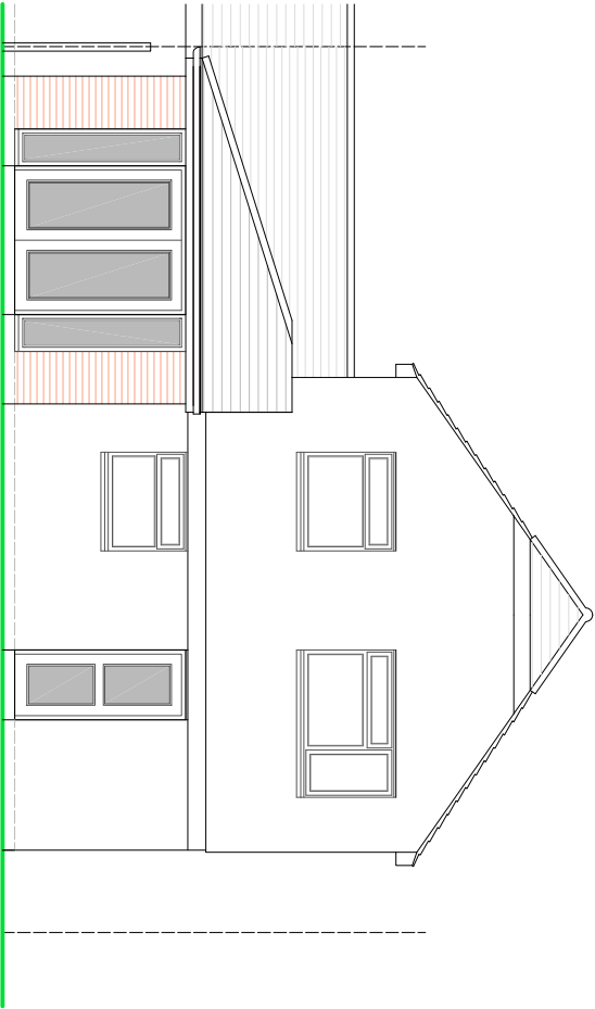
REAR ELEVATION
