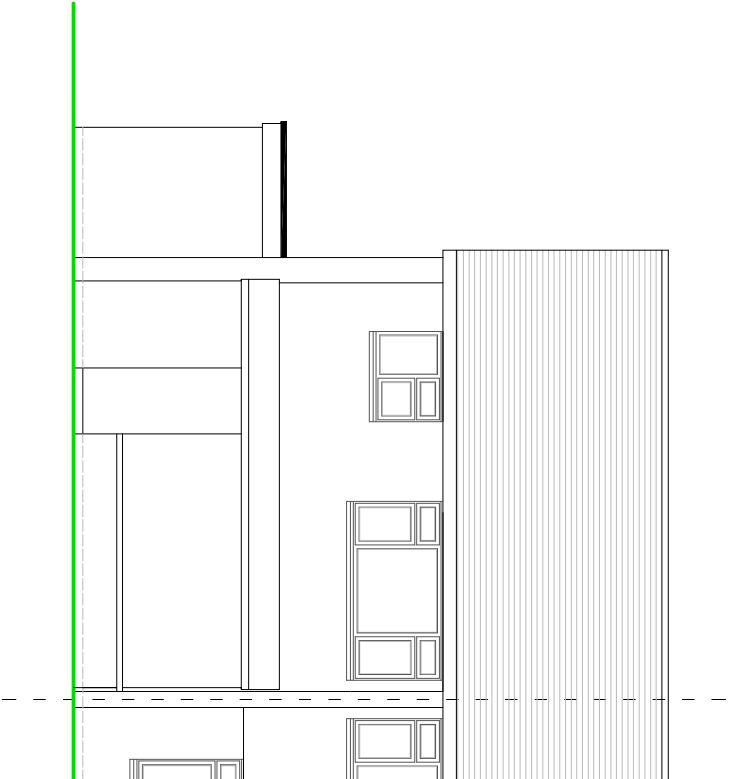
REAR ELEVATION
