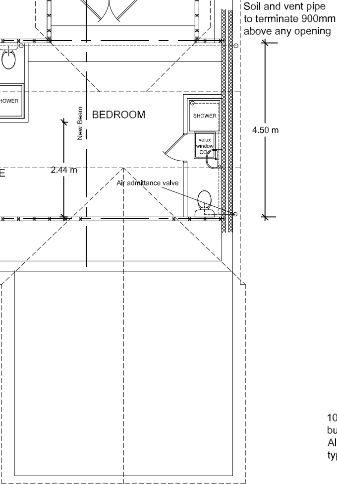
NEW ROOF PLAN
