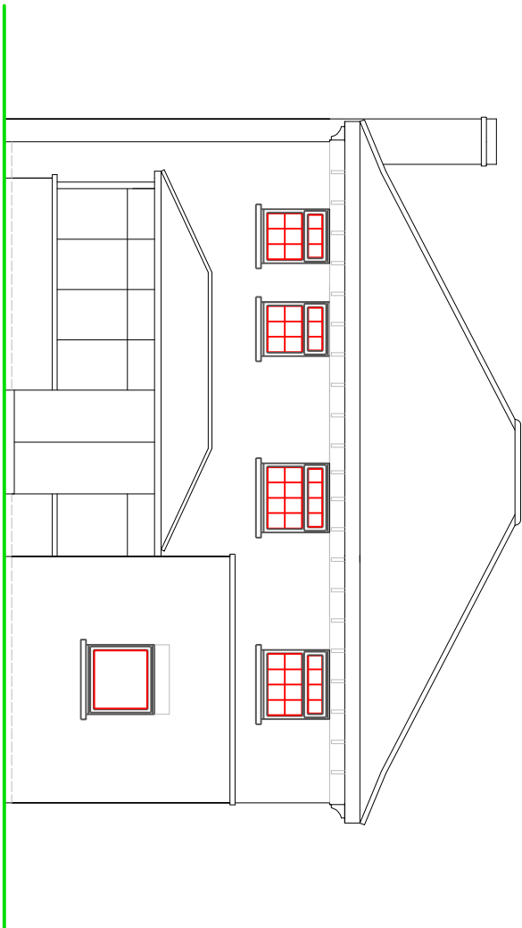
REAR ELEVATION
