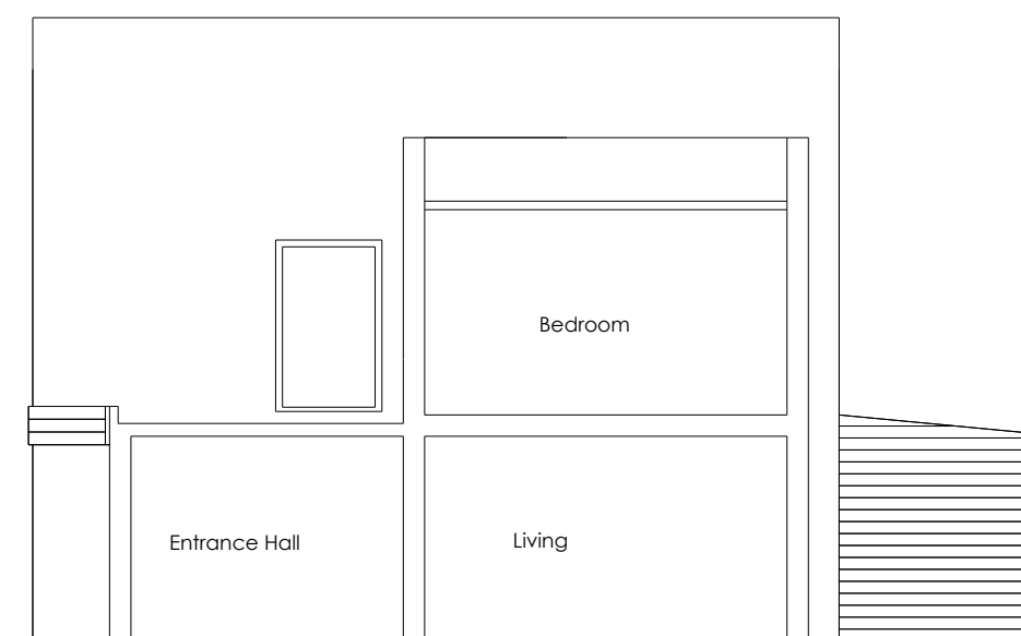
EXISTING CROSS SECTION B - B
