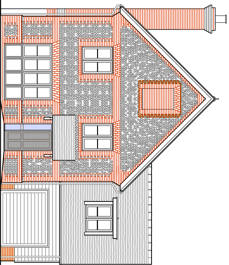
front elevation
