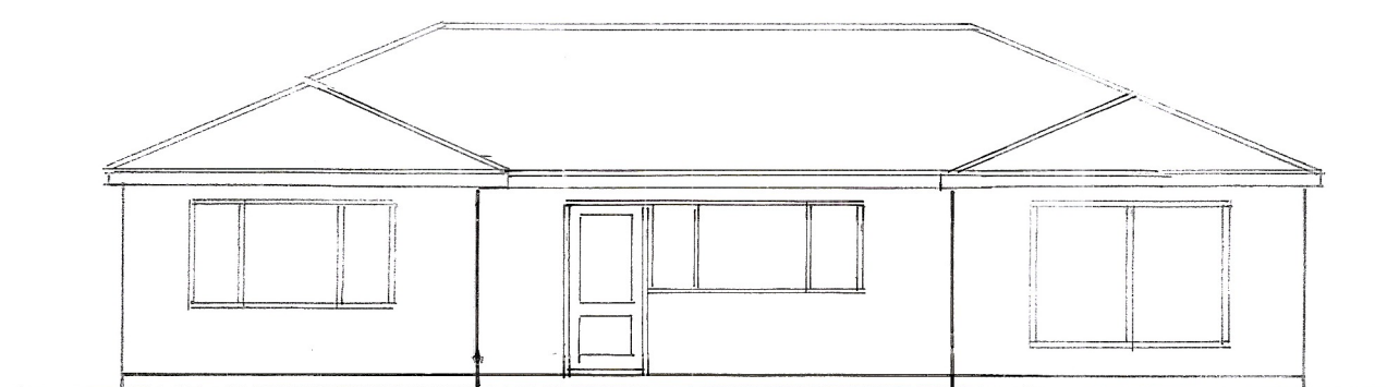
south 1:100
