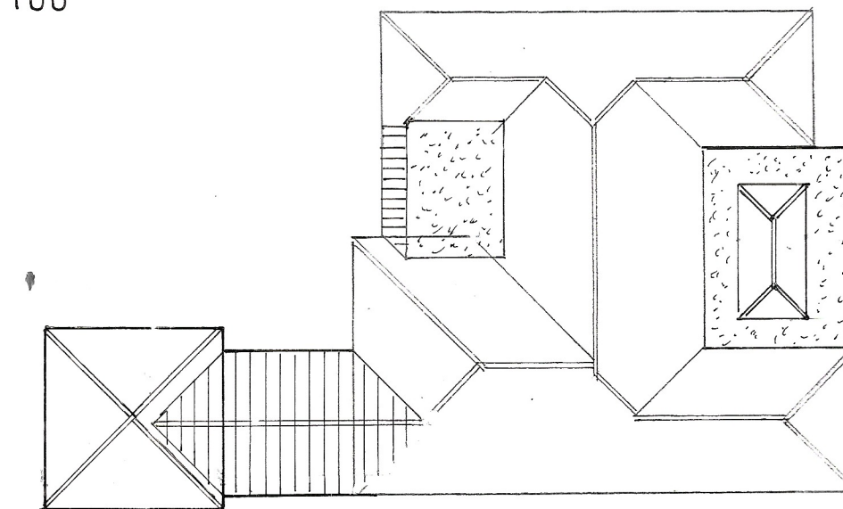
roof plan
