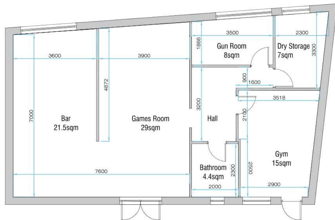
1 Existing floor plan 01 1:100
