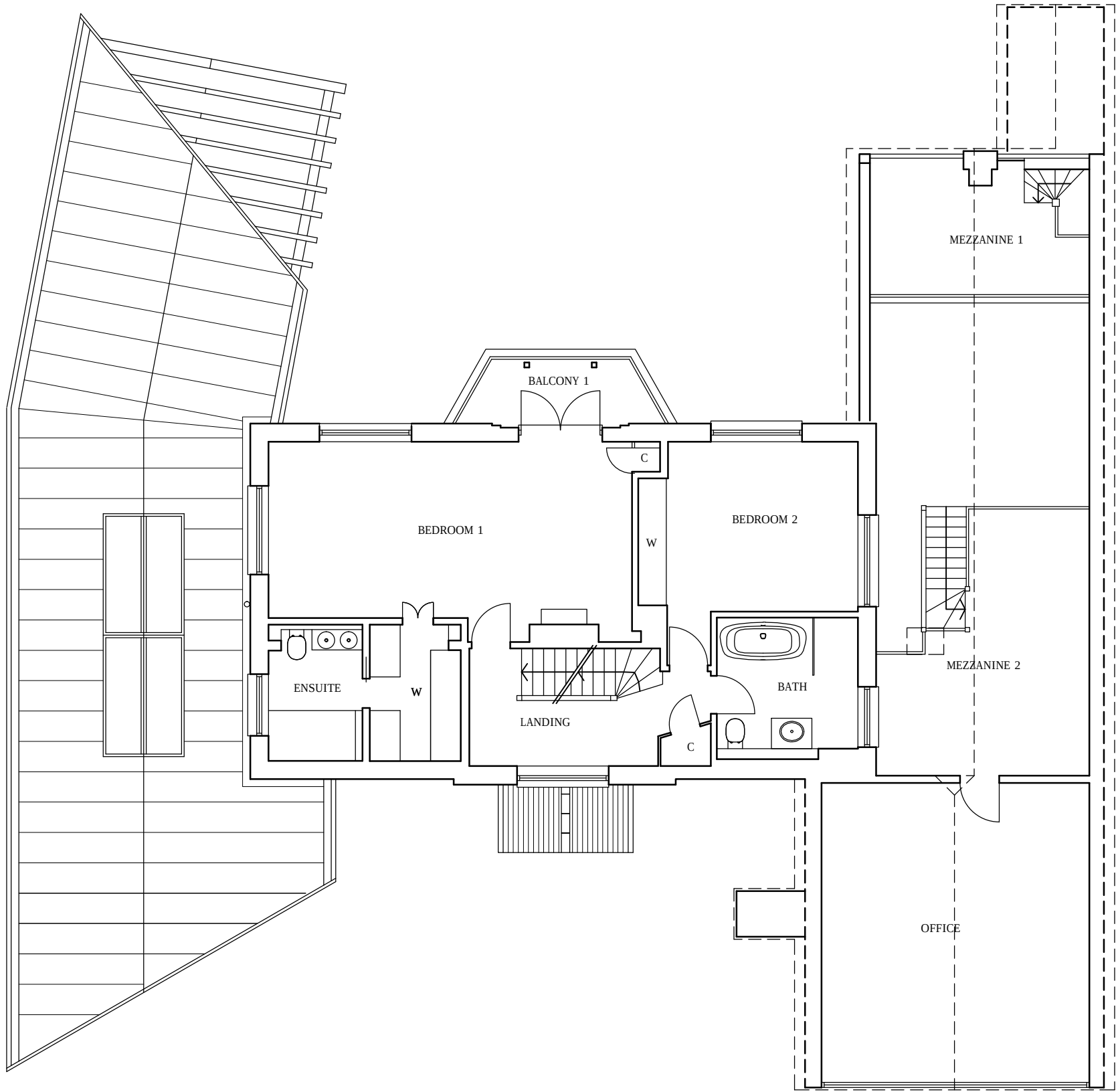
FIRST FLOOR
