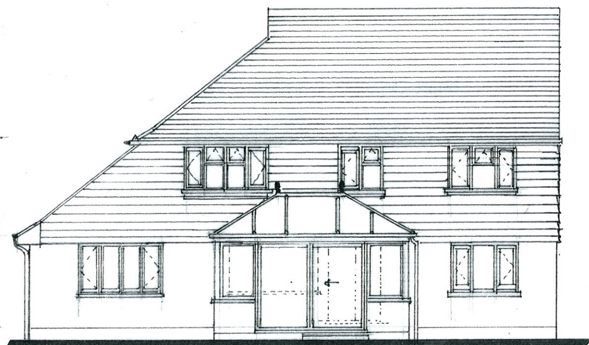
EXISTING ELEVATION REAR (UNCHANGED)
