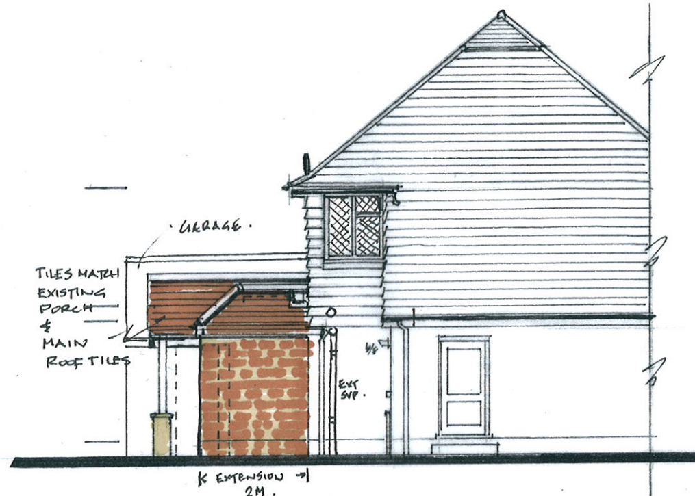
PROPOSED SIDE (RH) ELEVATION.
