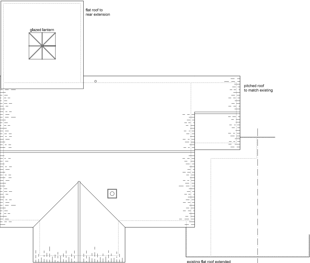
Roof Plan
