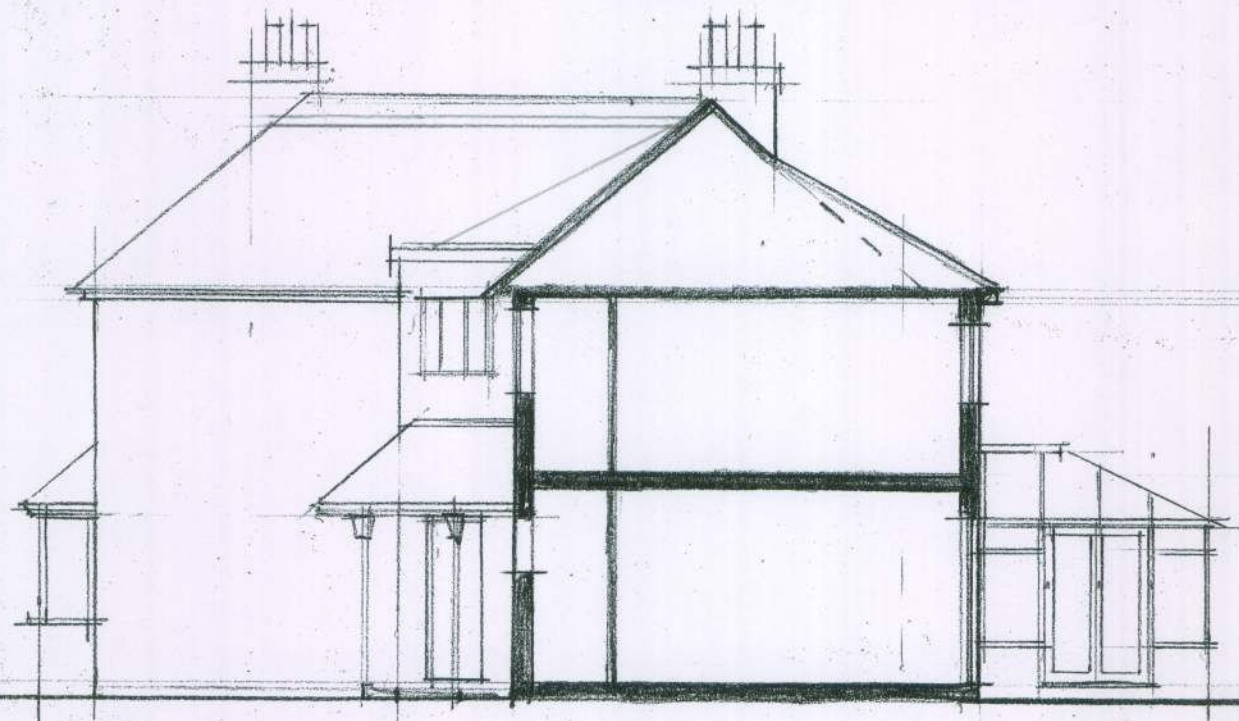
CROSS SECTION (LOOKING SOUTH)
