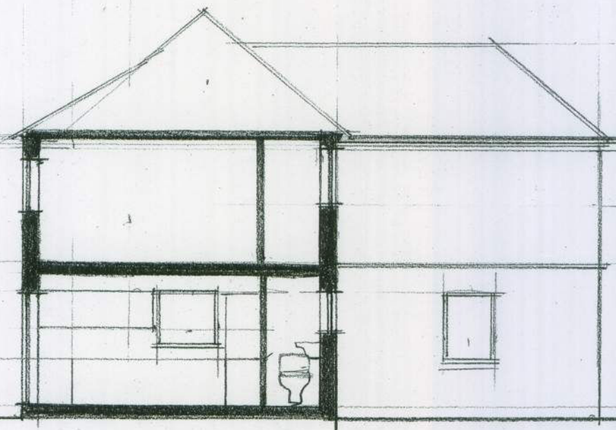
CROSS SECTION (LOOKING NORTH)
