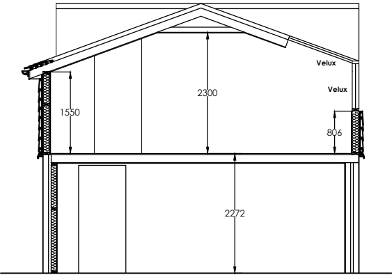
SECTION A
