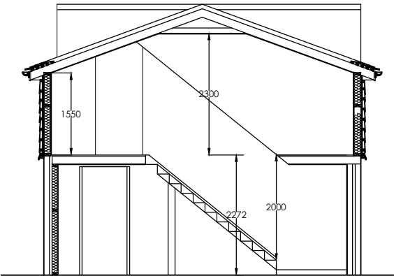
SECTION B
