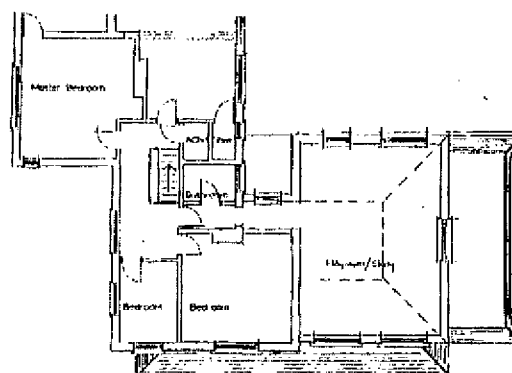
PROPOSED FIRST FLOOR PLAN (part)
