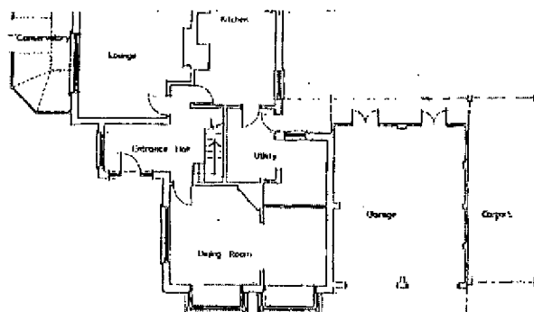
PROPOSED GROUND FLOOR PLAN (part)
