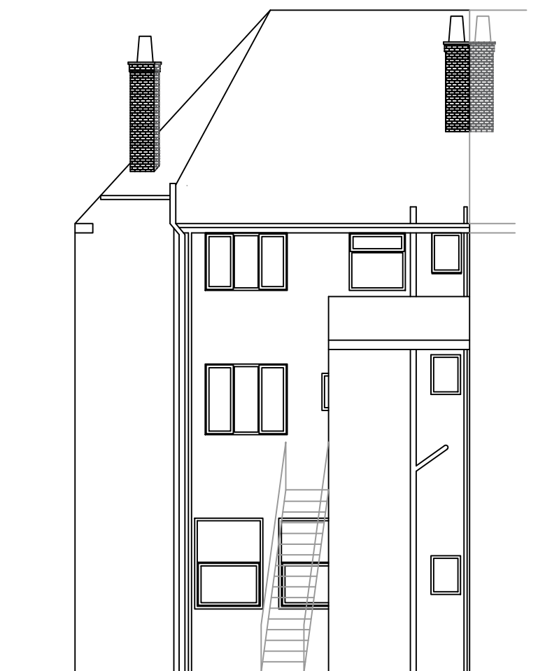
SOUTH (REAR) ELEVATION
