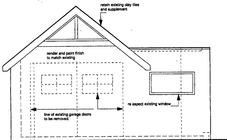
WESTERN ELEVATION
